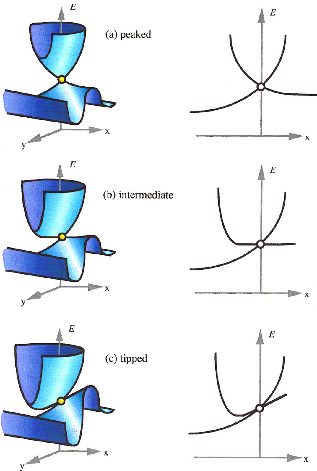
Figure 1.5 3D and 2D representations of the three different types of conical intersection.
